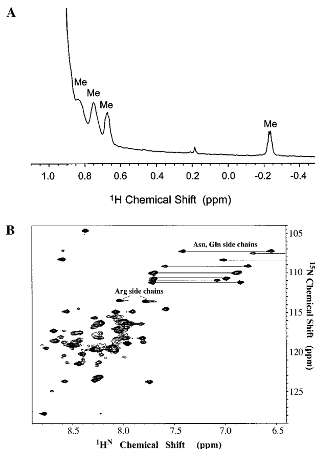
FIGURE 6: NMR spectra of wild-type ImmE1. (A) Upfield region of the ^1\text{H} NMR spectrum of ImmE1 (50 \mu\text{M} ) in 4:4:1 \text{CDCl}_3/\text{CD}_3\text{OH}/\text{H}_2\text{O} . Several methyl resonances, labeled at -0.25, 0.67, 0.76, and 0.82 ppm, are shifted upfield from the approximate position of 0.9–1.15 ppm associated with unshifted methyl groups of aliphatic residue side chains, reflect long-range contacts with aromatic side chains elsewhere in the protein and are indicative of a stably folded structure. (B) Two-dimensional ^1\text{H}/^{15}\text{N} HSQC NMR spectrum (600 MHz) of uniformly ^{15}\text{N} -labeled ImmE1 protein (0.3 mM) in 4:4:1 \text{CDCl}_3/\text{CD}_3\text{OH}/\text{H}_2\text{O} . The amide protons show the limited chemical shift dispersion typical for membrane proteins (12, 13), consistent with both a highly helical structure as well as the folded helical structure of a membrane protein. About 95 of the expected 109 backbone amide cross-peaks can be resolved when the spectrum is expanded 5-fold (not shown).
