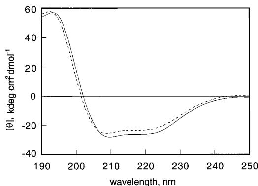
FIGURE 2: Far-UV circular dichroism spectrum of wild-type ImmE1. The purified ImmE1 was solubilized in 1-butanol/H 2 O, 19:1 v/v (solid), or 50% TFE (dashed). The secondary structure content, inferred from the analysis of the far-UV CD spectra in 1-butanol or TFE, was \alpha -helix, 79 or 77%; \beta -sheet, 10 or 9%; \beta -turns, 3 or 3%; remainder, 8 or 10%, respectively.
