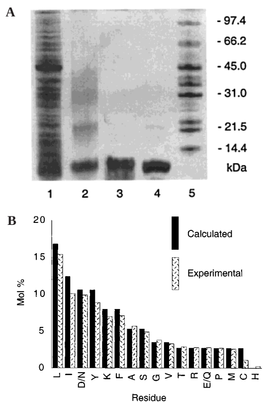
FIGURE 1: Extraction, purification, and identification of ImmE1. (A) Protein detected by silver staining following separation on a 12.5% SDS–polyacrylamide gel. Lane 1, isolated membranes following extraction with 2 M NaBr; lane 2, organic phase following butanol extraction of NaBr washed membranes; lane 3, pooled fractions following Sephadex LH 20-100; lane 4, pooled fractions following CM-cellulose; lane 5, low molecular weight protein standards. (B) Comparison of ImmE1 amino acid composition calculated from the primary sequence (solid bars) with that determined for pooled fractions following CM-cellulose (hatched bars).
