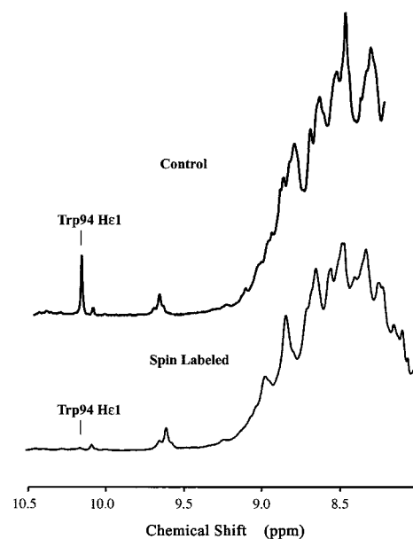
FIGURE 7: Broadening of indole NH region of Trp94 by spin label adduct of Cys16. Upper panel: Control, showing the indole H-1 of the Trp94 ImmE1 mutant. Lower panel: PROXYL-modified Cys50Ala/Cys94Trp ImmE1, showing the loss of the indole spectrum in the presence of PROXYL-modified Cys16. The extent of the relaxation effect indicates that the nitroxide radical attached to Cys16 and the Trp94 indole side chain are within 10–15 Å of each other.
