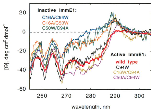
FIGURE 5: CD spectra of wild-type and mutant ImmE1 in the near-UV region. Spectra were taken in a chloroform/methanol/H 2 O (4:4:1) solvent system at 23 °C of ImmE1 mutant proteins in which Cys at positions 16, 50, and/or 94 were substituted to Ala and/or Trp. Spectra of wild type (bold red), C94W (black), C16A/C94W (blue), C16A/C50W (orange), C16W/C94A (brown), C50A/C94W (violet), and C50W/C94A (green) ImmE1 are shown.
